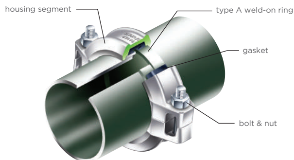
#S35 shouldered coupling
