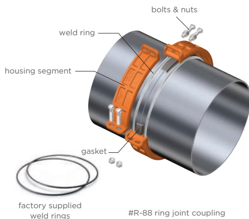
#R-88 ring joint coupling
