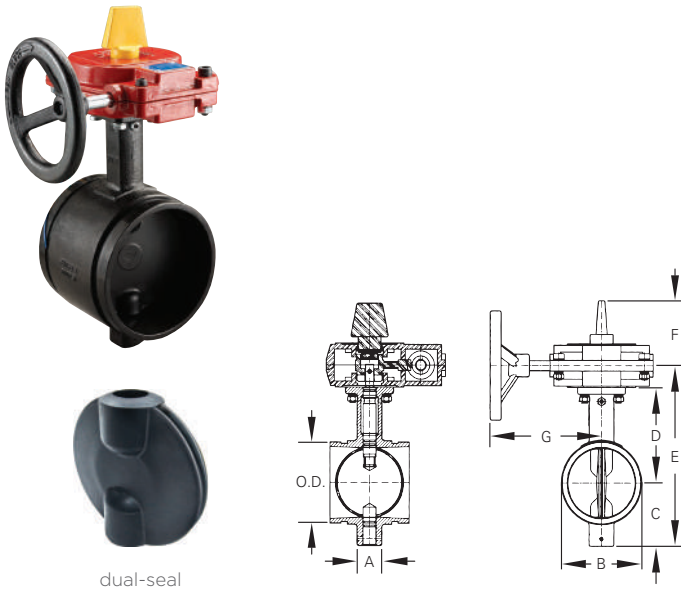
dual-seal
